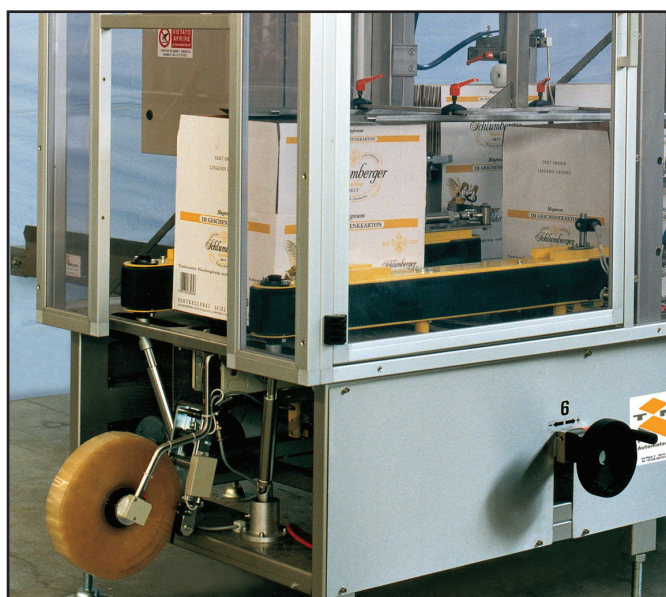
Adhesive taping unit with end of roll and tape-break signal.
